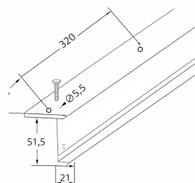
1 Perfil corredora superior Top runner profile
