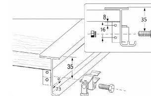
3 Freno soporte superior Top stop support
