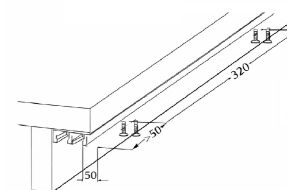
2 Perfil corredora inferior Bottom runner profile
